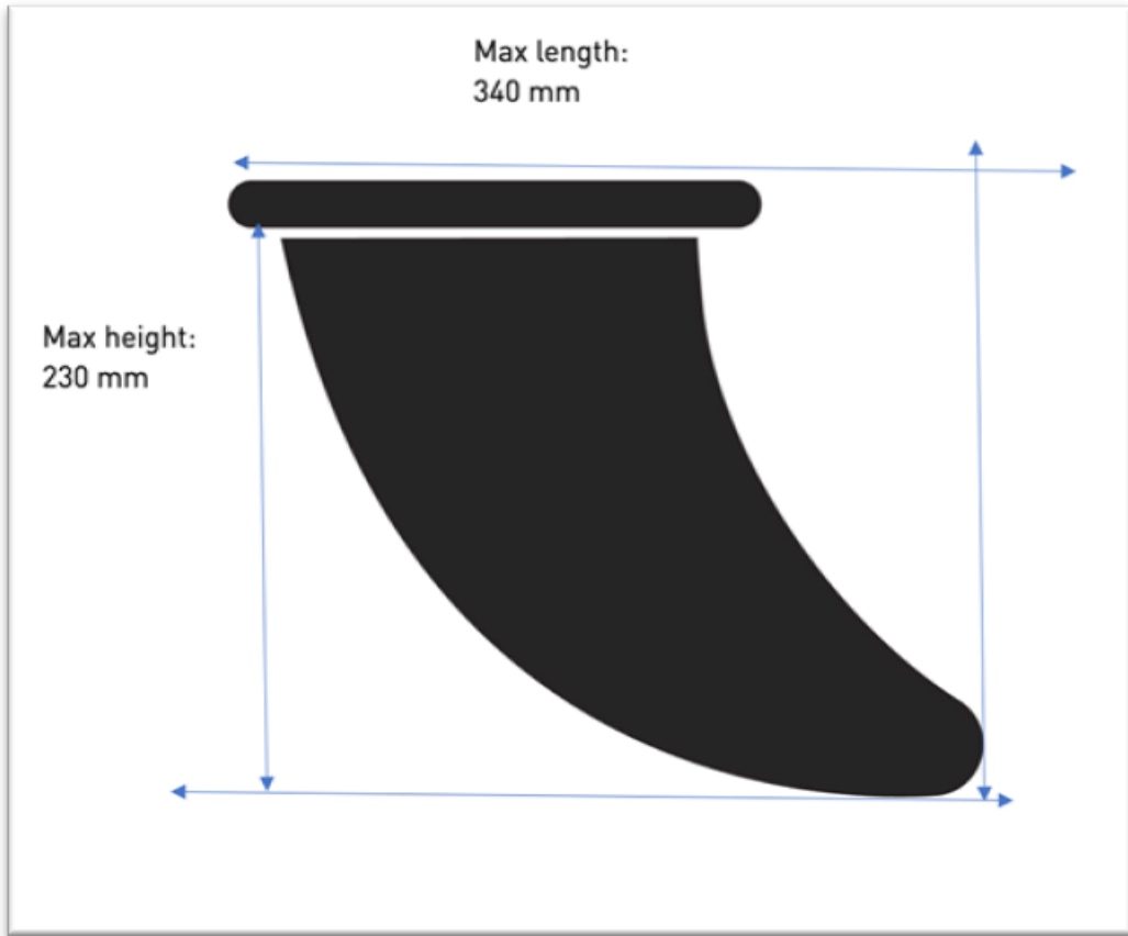
Picture 2 – Main fin scheme:
